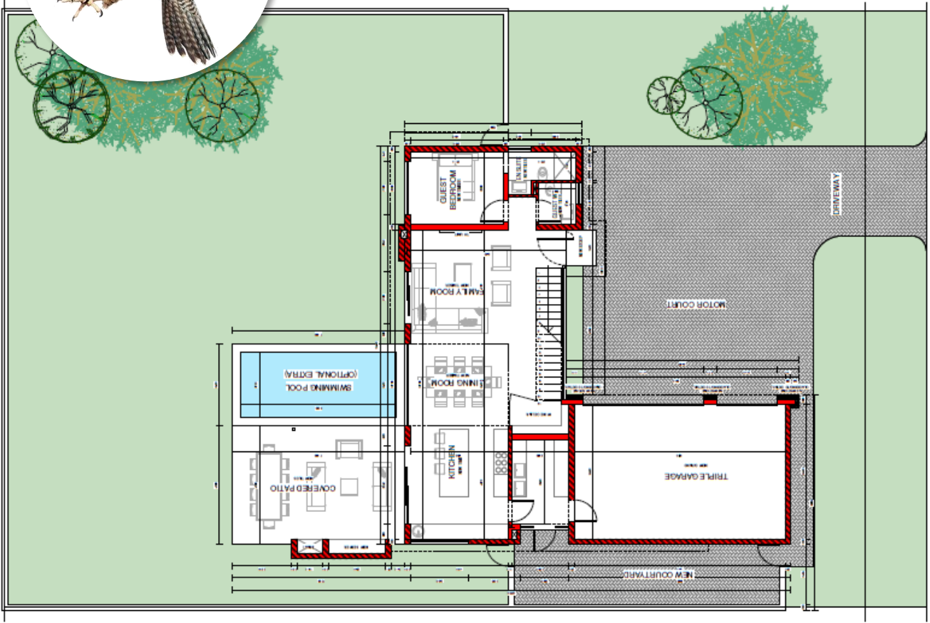
GROUND FLOOR LEVEL_HOUSE 3 1:50
